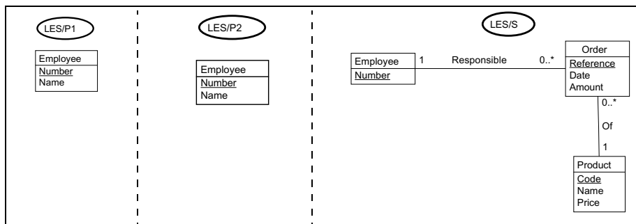
Fig. 9. The local extracted schemas. In LES/P1, the entity type PERSON is renamed EMPLOYEE (distance reduction) and only the attributes NUMBER and NAME are kept. LES/P2 comprises only the entity type EMPLOYEE and its attributes NUMBER and NAME. LES/S contains all the structures of LCS/S.
