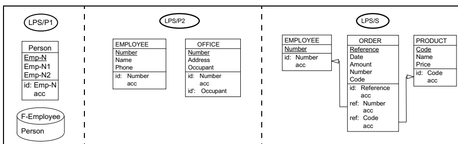
Fig. 5. The local physical schemas. LPS/P1 is made of one file (F-EMPLOYEE) and one record type (PERSON). EMP-N is a unique record key. LPS/P2 comprises the tables EMPLOYEE and OFFICE. LPS/S comprises three tables EMPLOYEE, ORDER and PRODUCT. Keys are represented by the id (primary) and id' (secondary) constructs, foreign keys by the ref construct + a directed arc, and indexes by the acc(ess key) construct.
