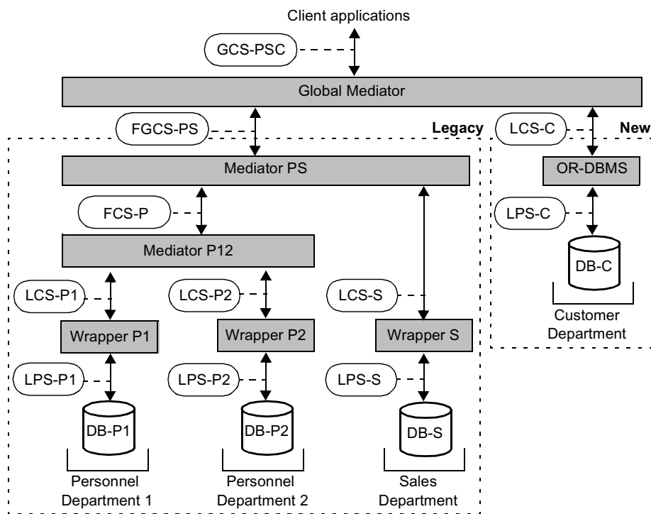
Fig. 1. The new system, available as a unique integrated database with schema GCS-PSC, will comprise a federated database that abstracts and integrates three independent legacy database (COBOL files DB-PP1, Oracle 5 DB-P2, DB2 DB-S), and the new object-relational database DB-C.
