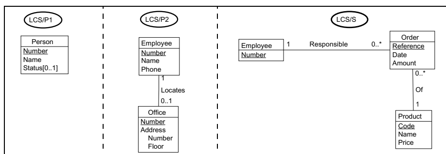
Fig. 6. The local conceptual schemas. In LCS/P, we observe the renaming and the elicitation of an implicit optional attribute. In LCS/P2, a hidden foreign key and an implicit compound attribute have been discovered. In LCS/P2 and LCS/S, the relational foreign keys have been transformed into associations.
