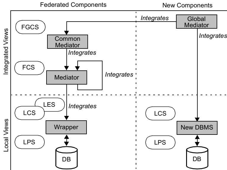
Fig. 2. Abstract model of the architecture.
