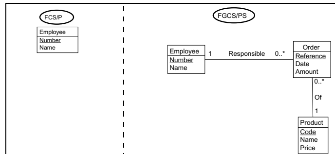
Fig. 11. The conceptual federated schemas. FCS/P integrates the LES of the personnel databases whereas FGCS integrates FCS/P and the LES of the sales department.
