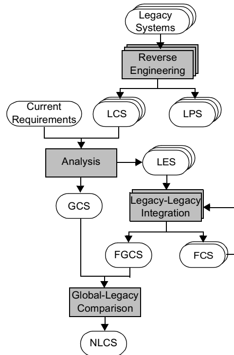
Fig. 3. The main processes of the methodology. The main product is the Global Conceptual Schema (GCS) that integrates the Federated Global Conceptual Schema (FGCS) and the New Local Conceptual Schema (NLCS) that describes the new database. Note that mapping definitions are ignored for simplicity.
