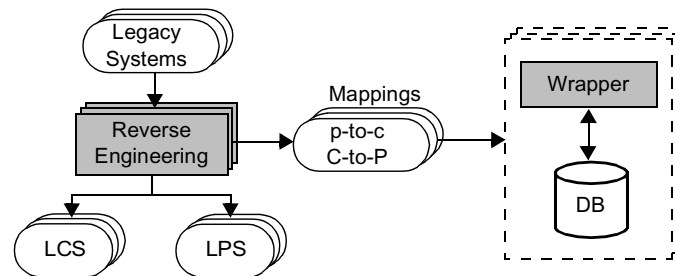
Fig. 4. Reverse engineering of the legacy databases.
