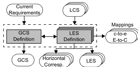
Fig. 7. The analysis process is made up of two subprocesses: the Global Conceptual Schema (GCS) definition and the Local Export Schemas (LES) definition.
