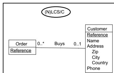
Fig. 13. The local conceptual schema of the new database.
