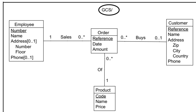
Fig. 8. The global conceptual schema that formalizes the requirements to be met by the future system.
