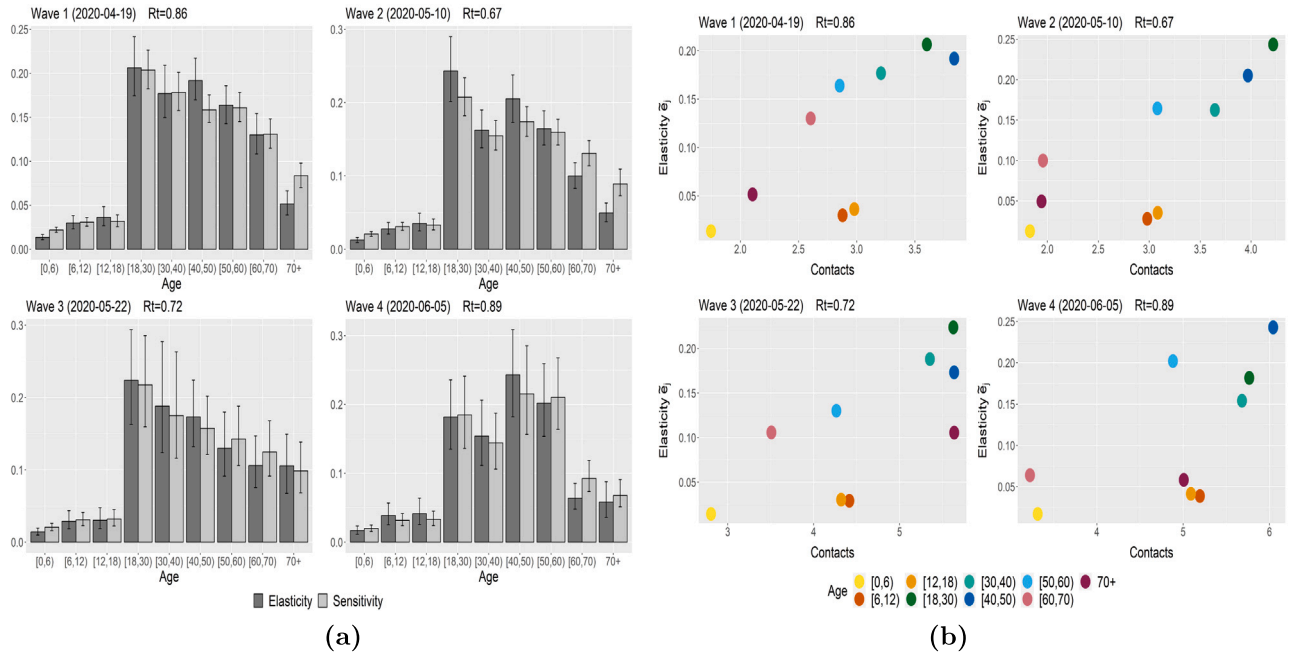
Fig. 3. Age-specific sensitivity and elasticity evolution over the period April–June 2020. Panel (a) represents the evolution of the cumulative indices \bar{s}_j and \bar{e}_j for all i, j = 1, \dots, n . The error bars reflect the 95% percentile interval obtained from 1000 bootstrap samples of the social contact matrices. Panel (b) consists of consecutive plots comparing cumulative contacts (x-axis) and cumulative elasticities (y-axis). The age groups in the top-right portion of the graphs contribute the most to transmission at the observation time. This corresponds to different CoMix survey waves (Coletti et al., 2020), for which we indicate the calendar time and the R_t obtained from Sciensano (2021).
