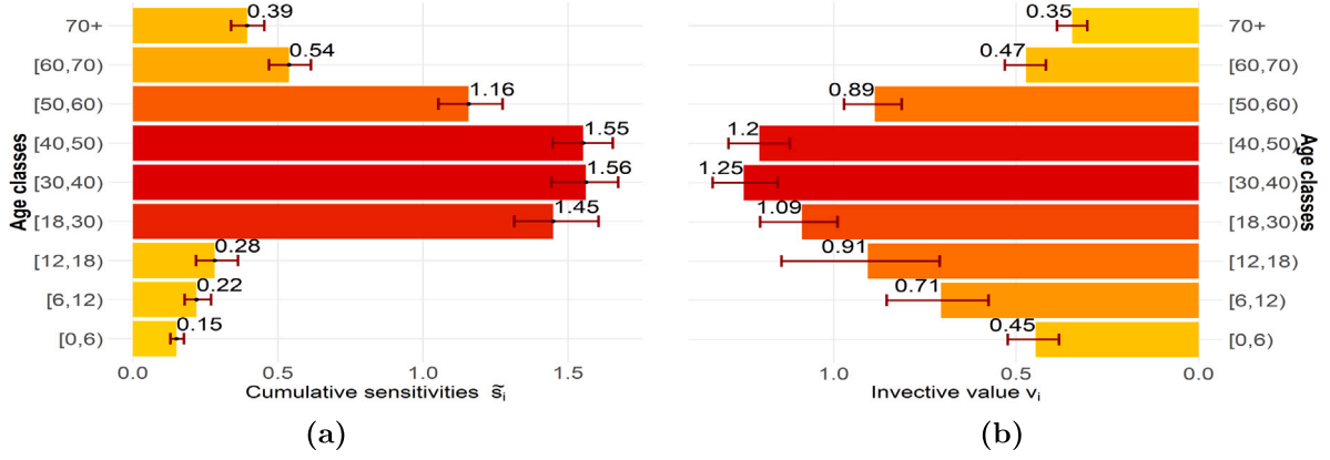
Fig. F.8. Panel(a): age-specific cumulative sensitivities \tilde{s}_i . Panel(b): infective value of a single infection in each age group. We show the 95% percentile interval obtained with 1000 bootstraps of the social contact data sample.
