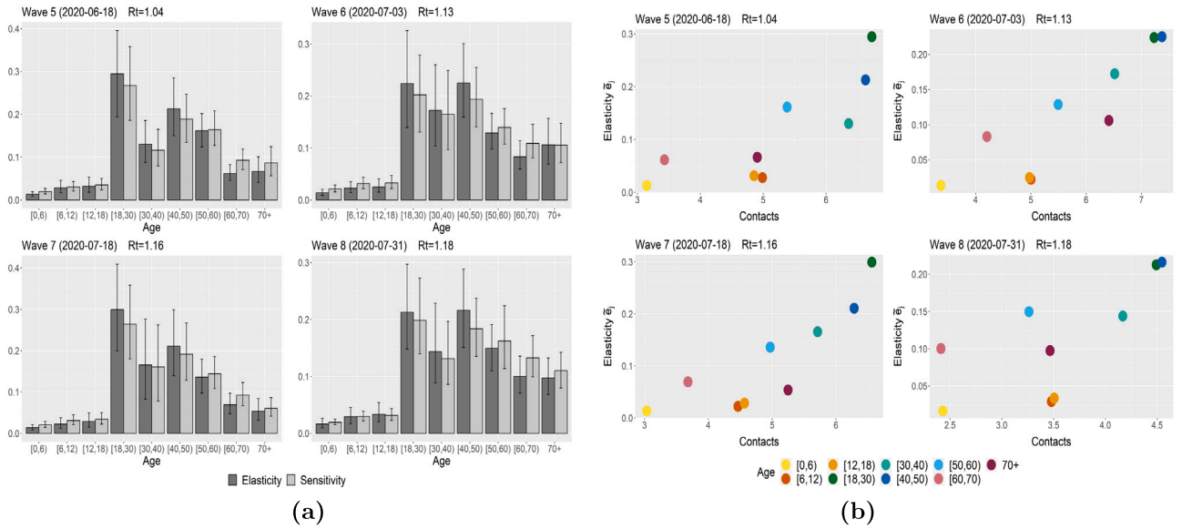
Fig. F.13. Age-specific sensitivity and elasticity evolution June–July 2020. Panel (a) shows the evolution of the cumulative indices \bar{s}_j , \bar{e}_j for all i, j = 1, \dots, n reported with the error bars as evaluated from 1000 bootstrap samples of the social contact matrices. Panel (b) consists of consecutive plots comparing cumulative contacts (x-axis) and cumulative elasticities (y-axis). The age groups in the top-right portion of the graphs contribute the most to transmission at the observation time. This corresponds to different CoMix survey waves (Coletti et al., 2020), for which we indicate the calendar time and the R_t obtained from Sciensano (2021).
