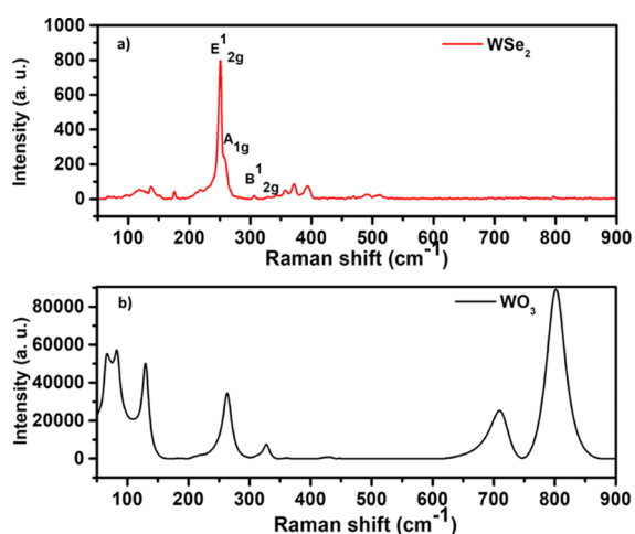
Figure 4. Raman spectra of (a) as-grown WSe 2 nanoflowered film and (b) WO 3 nanowires.
