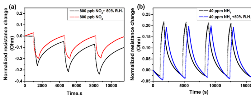
Figure 11. Dry and relative humidity cross-sensitivity to (a) 0.8 ppm NO 2 at 100 °C and (b) 40 ppm NH 3 at 150 °C.
