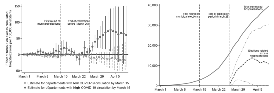
Fig. 7 Estimates using up to 14 days after the end of the calibration period. Sub-figures (a) and (b) mimic Figs. 2 and 3, but use observations up to 14 days after March 26. Vertical lines are 95% confidence intervals. Short dashed lines are bounds of 95% confidence intervals
