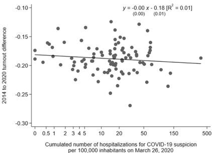
Fig. 1 Electoral turnout and the COVID-19 epidemic. Sources: Authors' calculation using Santé publique France, Ministère de l'intérieur and Institut national de la statistique et des études économiques data. Regression lines of each sub-figure represent the linear relationship between the variable represented on the y-axis and the variable represented in the x-axis. Associated equations displays estimated coefficients and their standards errors (in parentheses)
