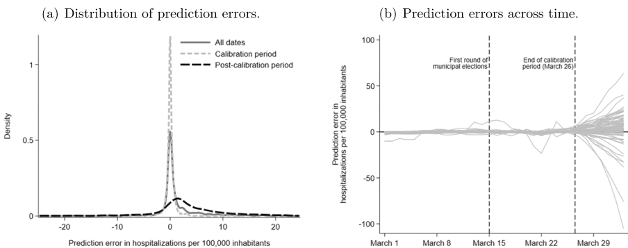
Fig. 9 Prediction errors. Sub-figures (a) and (b) plot the prediction errors of model Eq. 1 calibrated until March 26. Predictions are computed up to 7 after the end of the calibration period. See Section 3 for more details. Figure (a) excludes prediction errors out of the [-25, 25] range
