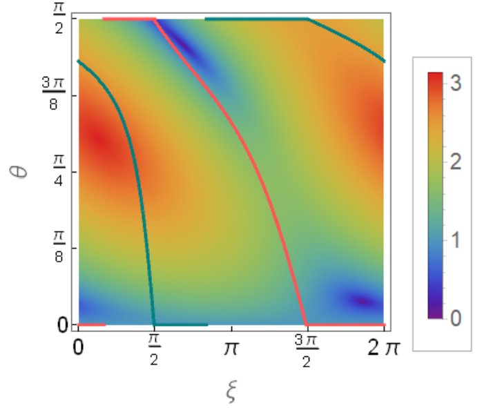
FIG. 3. Color map of the angle between the vectors representing the post-selected state on the Bloch sphere \vec{f}_1 and \vec{f}_2 as a function of \theta and \xi . The red line represents the angle \theta for which the modulus of the weak value is maximum for fixed values of \xi , \theta_{\max}(\xi) . The green line represents the angle \theta for which the modulus of the weak value is minimum for fixed values of \xi , \theta_{\min}(\xi) .
