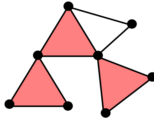
Simplicial complex (group interactions)
