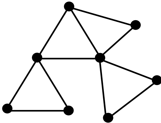
Network (pairwise interactions)
