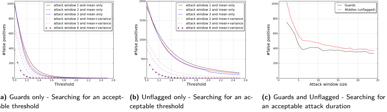
Fig. 7. OnionShape's result over December 2016 network history. We measure the average false positives for varying parameters to answer research questions of 4.4.1. Figure 9 complete this result by showing the variance of these measurements.
