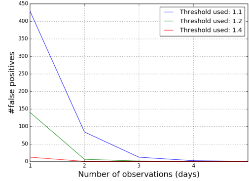
Fig. 12. Confidence of the adversary on multiple observations
