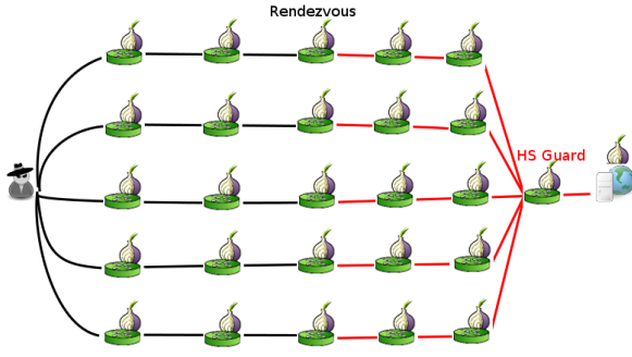
Fig. 3. Guard discovery technique: relay drop attack against an onion service. Black links are built by the adversary. Red links are built by the onion service.
