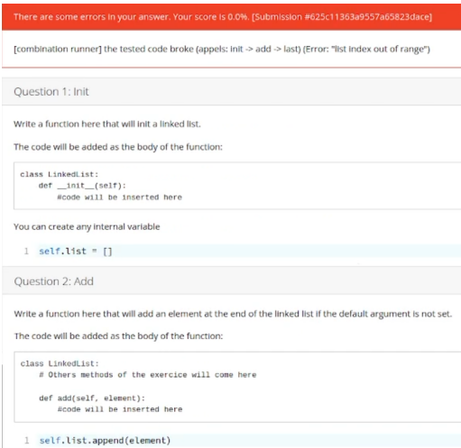
Figure 2: Example of usage of SIMPyTEST in INGINIOUS for a data structure definition (a list)
