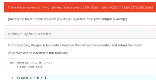
Figure 1: Example of usage of SIMPYTEST in INGINIOUS for a simple algorithmic problem (the addition of two integers)
