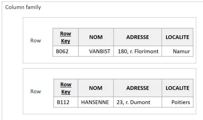
FIGURE 1.9 – Column-Family [Sad13]
