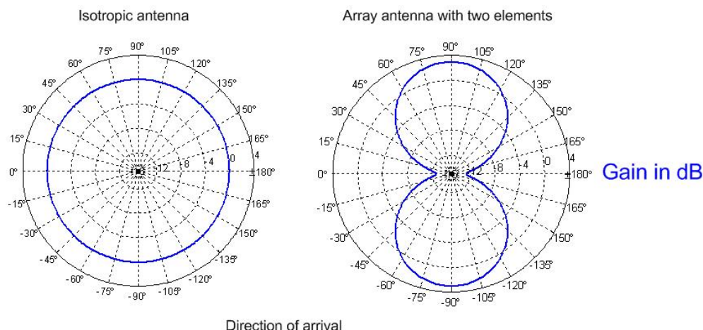
Figure 2.25: Radiation pattern
