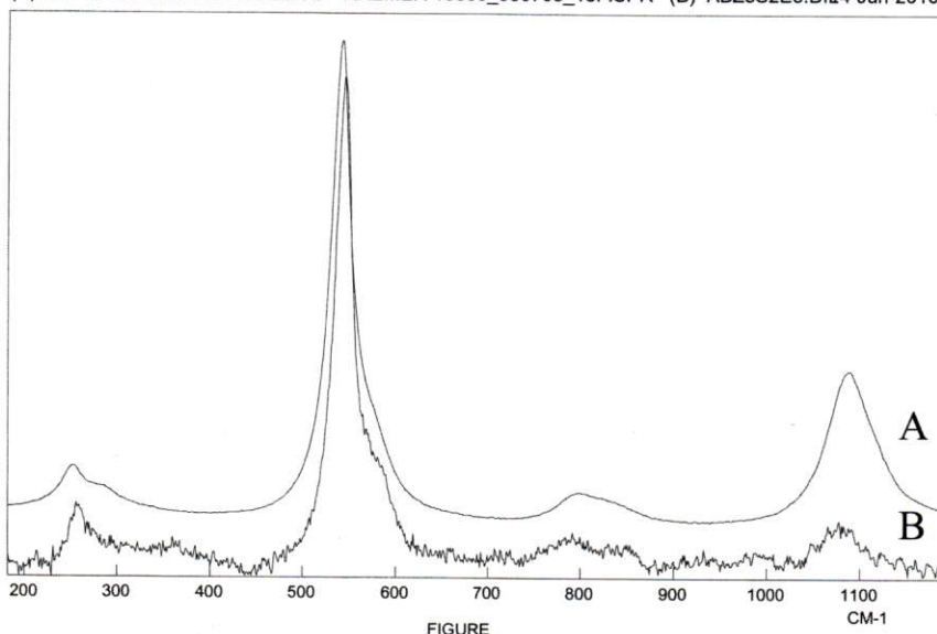
(A) LAPIS LAZULI FRA ANGELICO - KREMER 10530_060705_13F.SPR (B) ABZ3S2E5.DII4-Jun-2010
