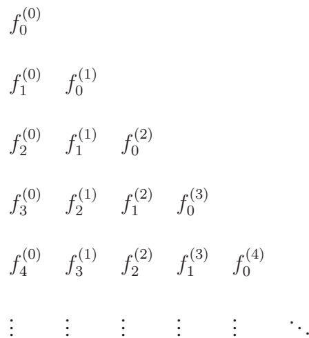
Figure F.1: Recursive transformation of an analytic function under Lie transform, better known as the Lie triangle
