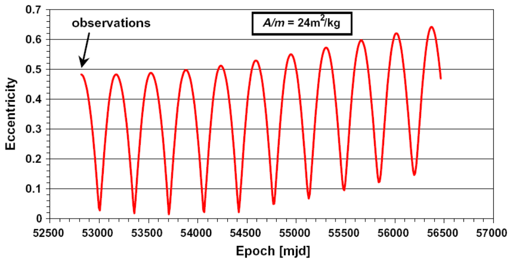
Figure 3.14: Evolution of the eccentricity for an object of the new population over ten years as computed in Schildknecht et al. (2007). The additional spurious long-periodic effect is clearly visible. [Graphic by Schildknecht et al. (2007)].
