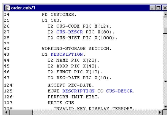
FIGURE 118. Example of variables belonging to the variable dependency graph shown in context.
