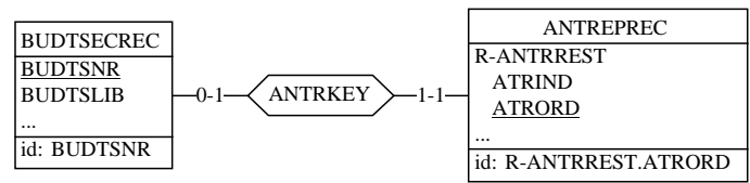
FIGURE 214. The conceptual schema.
