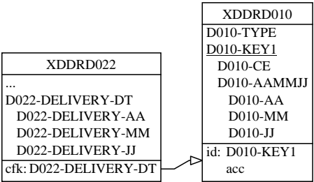
FIGURE 204. The complete logical schema.
