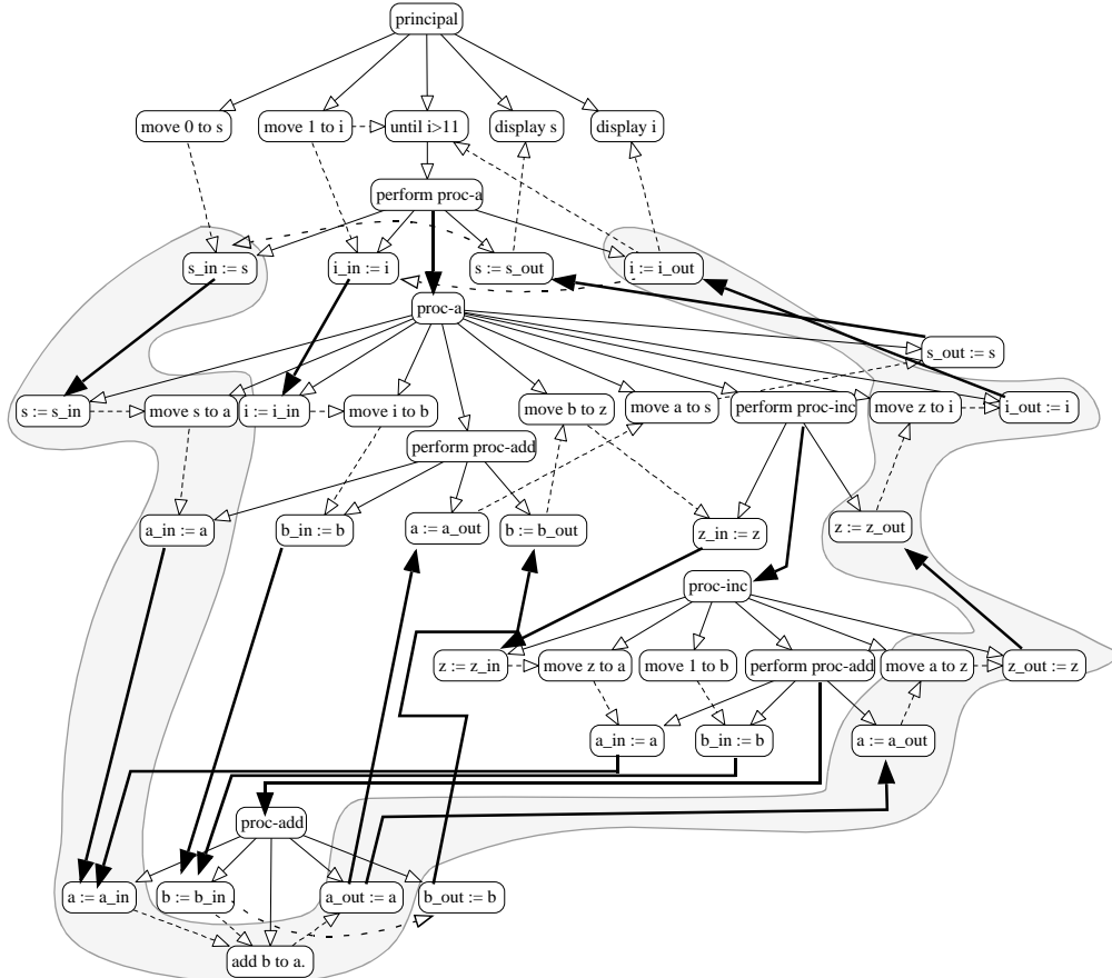
FIGURE 68. A program and its corresponding SDG. The PDG are connected with parameter-in, parameter-out and call edges.
