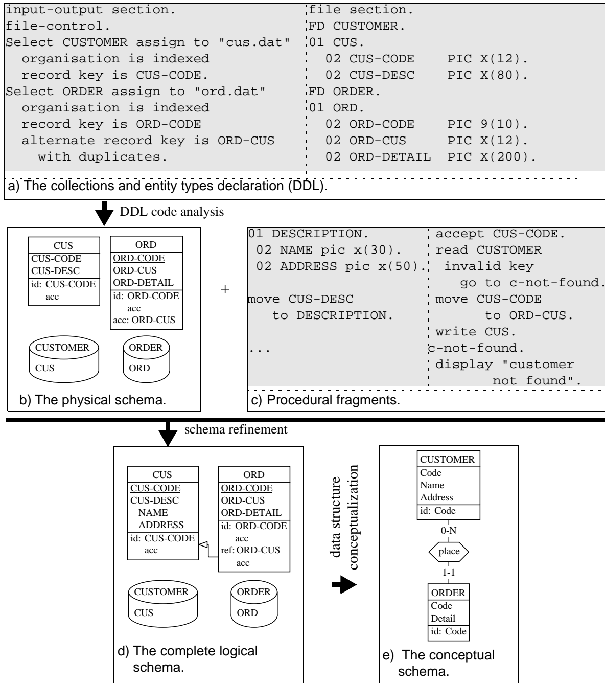
FIGURE 28. Database reverse engineering example.
