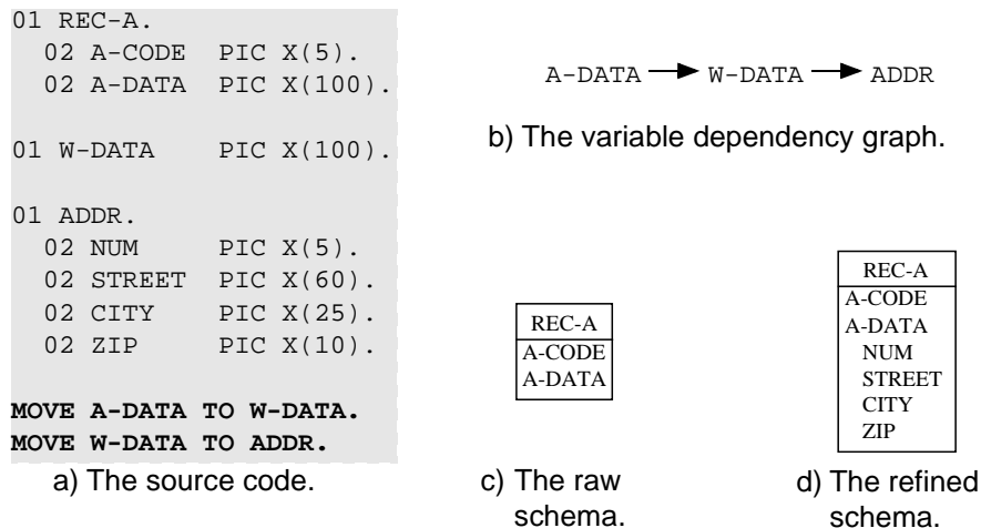
FIGURE 102. Example of attributes decomposition.
