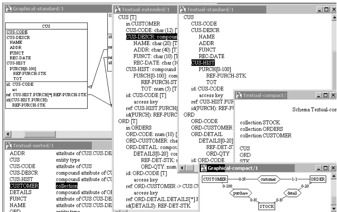
FIGURE 109. The six different extended entity-relationship views offered by DB-MAIN.
