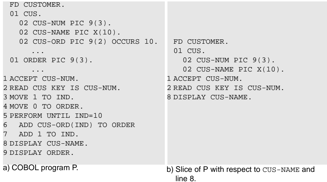
FIGURE 46. Example of program slice.
