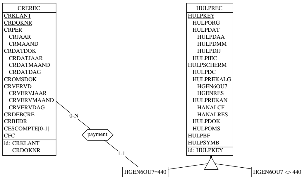
FIGURE 224. The conceptual schema.
